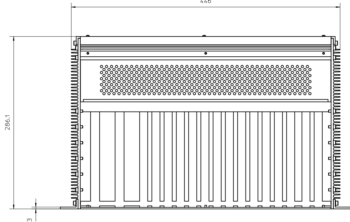
Top-view down without cover-plates
