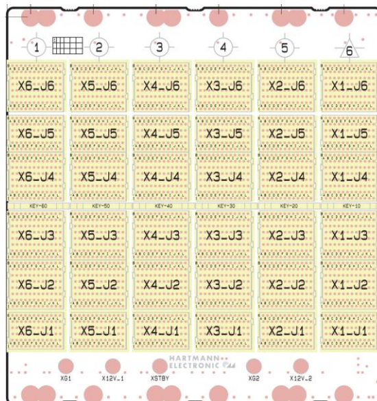
Front side
