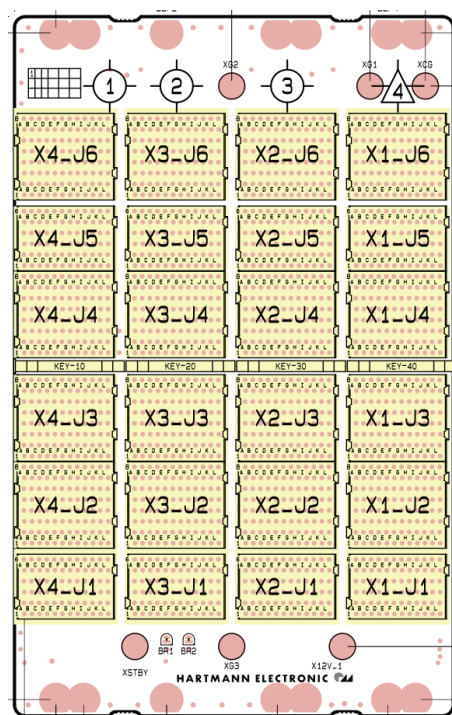
Front side
