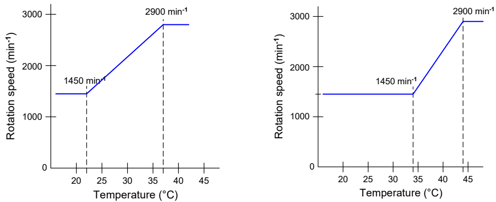
Figure 3-9 Fan characteristic dip-switch on/off
