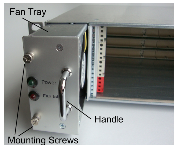
Figure 5-1 Fan Tray Components (sample: 2U version)
